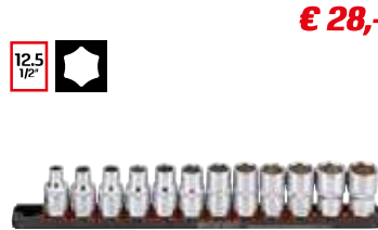
Art. nr 301201 Rack de douilles 1/2" courtes 6p, 12-pcs - 8, 9, 10, 11, 12, 13, 14, 15, 16, 17, 18, 19mm
